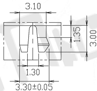
DETAIL X
