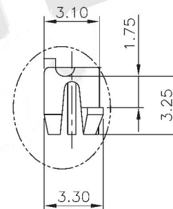
DETAIL Z SCALE 2:1
