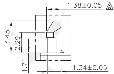
DETAIL X SCALE 4:1
