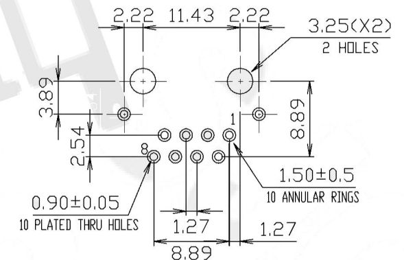
PC Board Layout REF.
