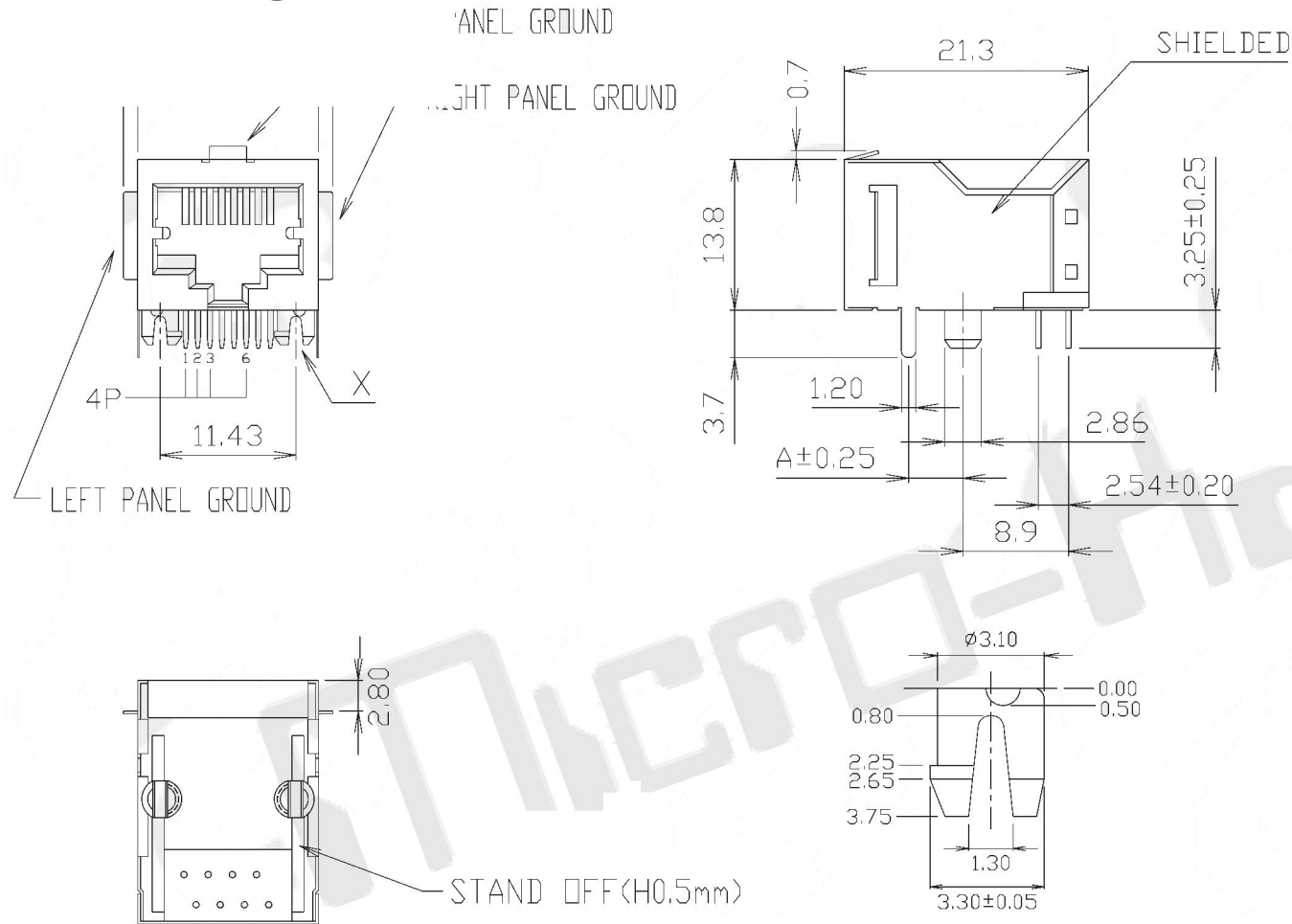
DETAIL X
