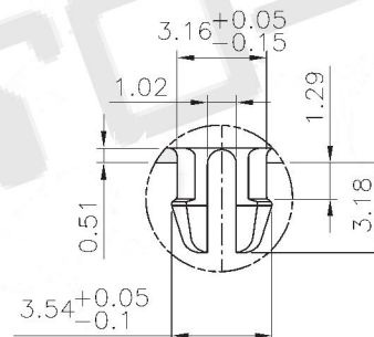
DETAIL Z SCALE 2:1
