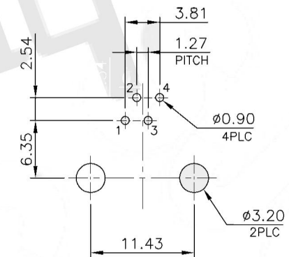
RECOMMENDED PCB LAYOUT PCB THICKNESS: 1.6mm TOLERANCE: ±0.05mm (TOP VIEW)
