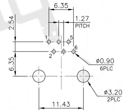
RECOMMENDED PCB LAYOUT PCB THICKNESS: 1.6mm TOLERANCE: ±0.05mm (TOP VIEW)
