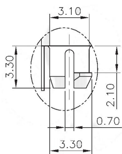
DETAIL Z SCALE 2:1
