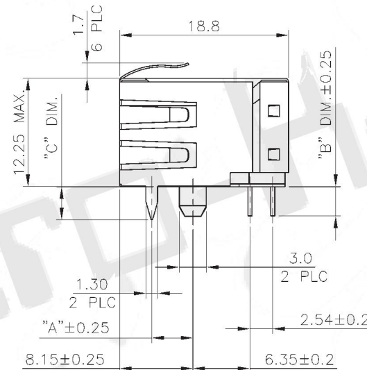
DETAIL Z SCALE 2:1
