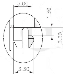
DETAIL Z SCALE 2:1
