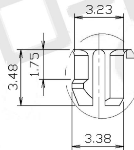
DETAIL X
