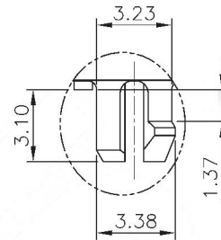
DETAIL Z SCALE 2:1
