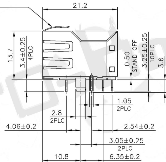
TOP PANEL GROUND (OPTIONAL)
