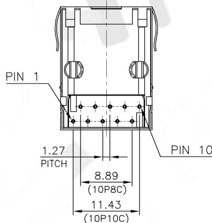
TOP & LEFT & RIGHT 3 SIDES WITH PANEL GROUND TYPE
