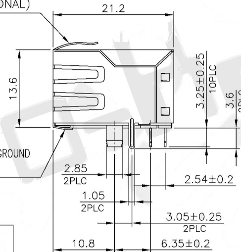
DETAIL Z SCALE 2:1
