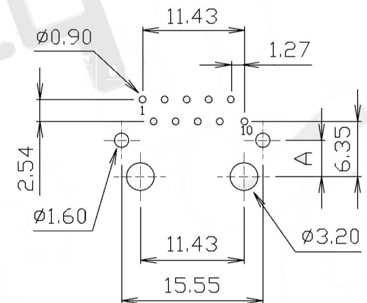
PC Board Layout DEC
