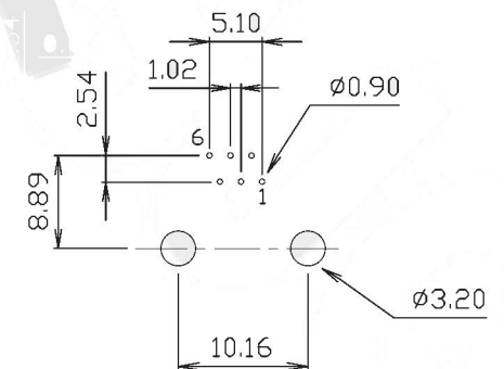
PC Board Layout Ref.
