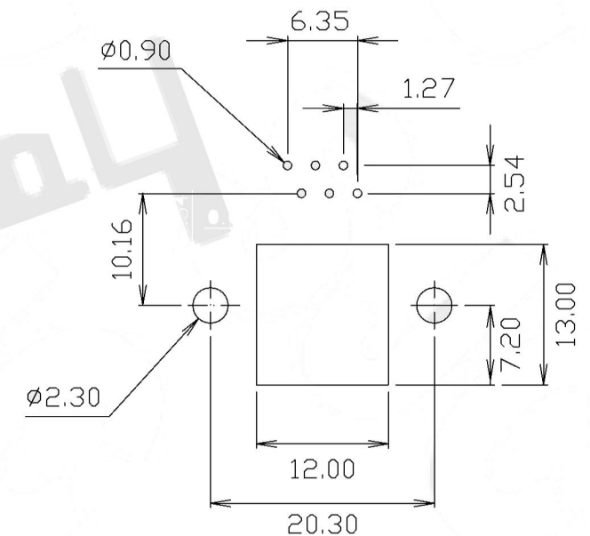
PC Board Layout
