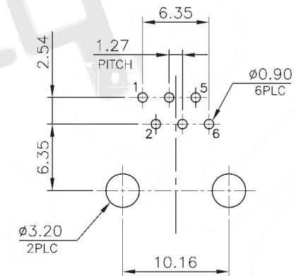
RECOMMENDED PCB LAYOUT PCB THICKNESS: 1.6mm TOLERANCE: ±0.05mm (TOP VIEW)
