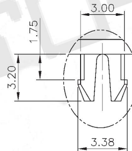
DETAIL Z SCALE 2:1
