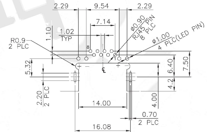
PCB LAYOUT Ref.
