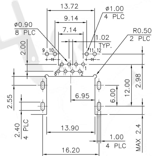
RECOMMENDED PCB JACK TOP VIEW
