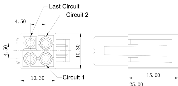
MR-C4500HF-2*02P
