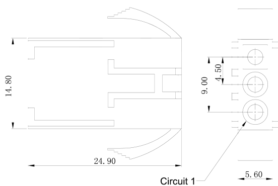
MR-C4500HM-3P
