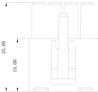
MR-C4500HF-4P
