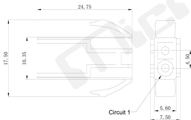
MR-C4500HM-2P
