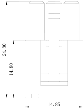
MR-C4500HF-3P
