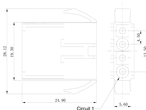
MR-C4500HM-4P
