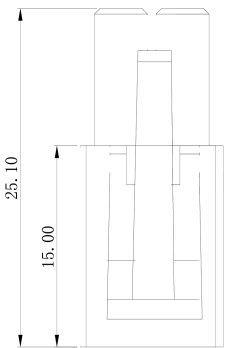
MR-C4500HF-2P
