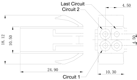
MR-C4500HM-2*02P
