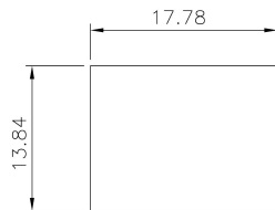
RECOMMENDED PANEL CUTOUT Ref.
