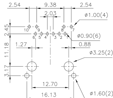
PCB LAYOUT Ref.
