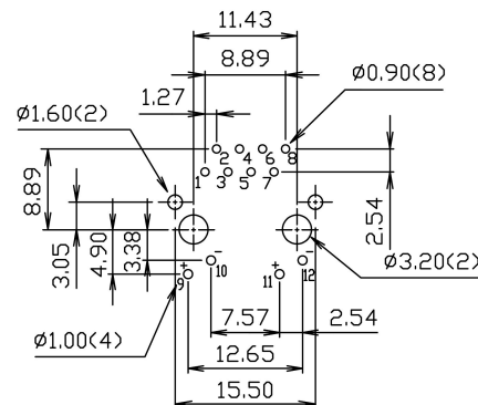
PC Board Layout Ref.
