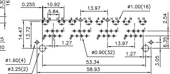
PCB LAYOUT Ref.
