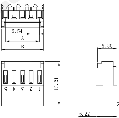
Feed- Thru Type With Polarizing Tabs
