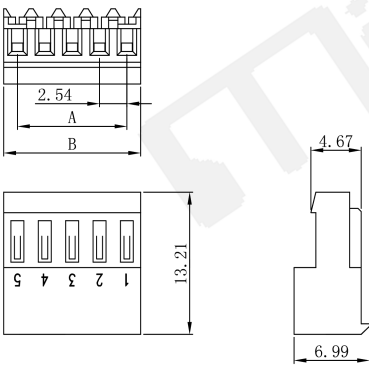
Closed End Type Without Polarizing Tabs
