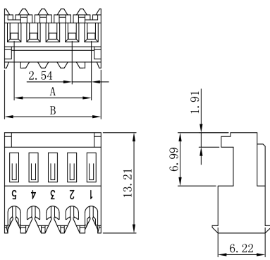
Feed- Thru Type With Polarizing Tabs
