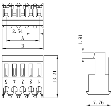
Feed- Thru Type Without Polarizing Tabs
