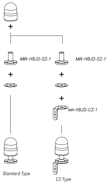
MR-HBJD-70 Installation Diagram
